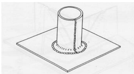
Pipe sleeve / lead slate
