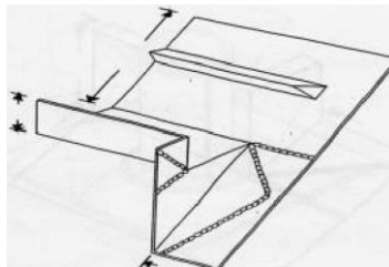
Back gutter
