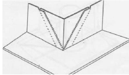
Gusset corner/ inclined welding
